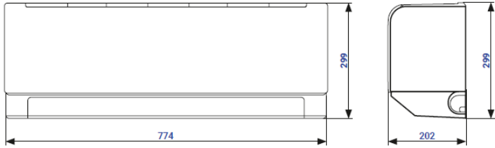
AUX-12CA
