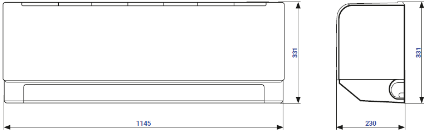
AUX-24C3A
