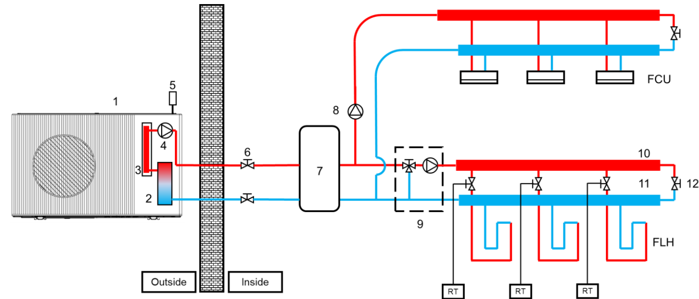
Figure 3.3.6: Space heating through floor heating loops and fan coil units
