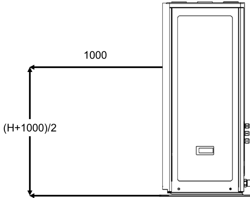
Monoblock sound pressure level measurement (unit: mm)
