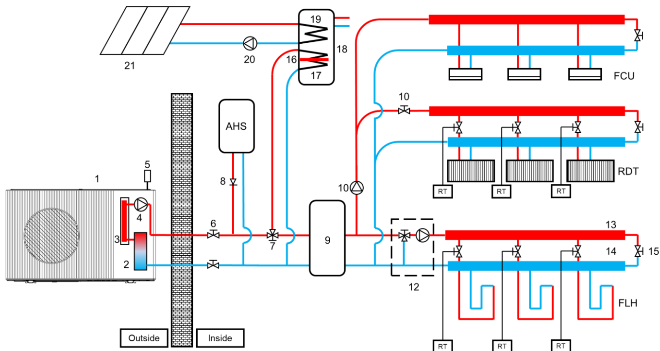
Figure 3.3.8 Space Heating with heat pump and AHS, space cooling with heat pump and solar for hot water
