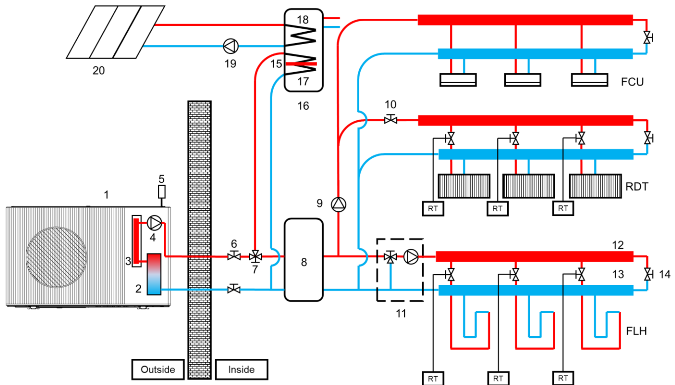
Figure 3.3.7 Space heating, space cooling and domestic hot water compatible with solar water heater
