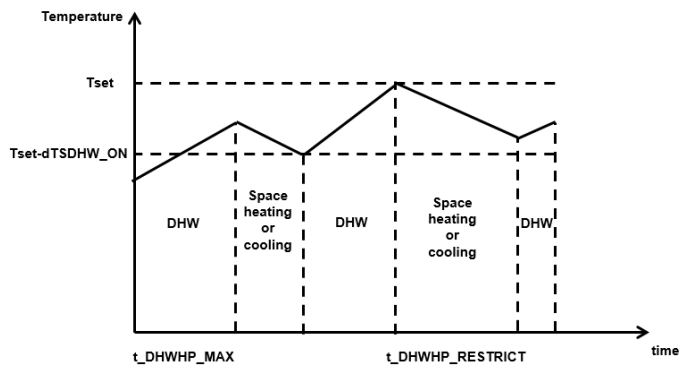
DHW PRIORITY
